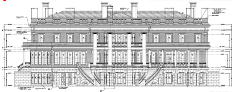
REAR EXTERIOR ELEVATION 1/2" = 1'-0"
